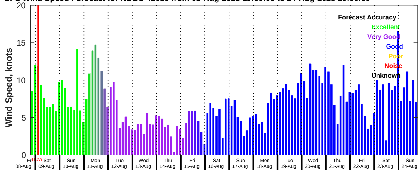
GFS Wind Speed Forecast for NDBC 42036 from 08-Aug-2025 19:00:00 to 24-Aug-2025 19:00:00
