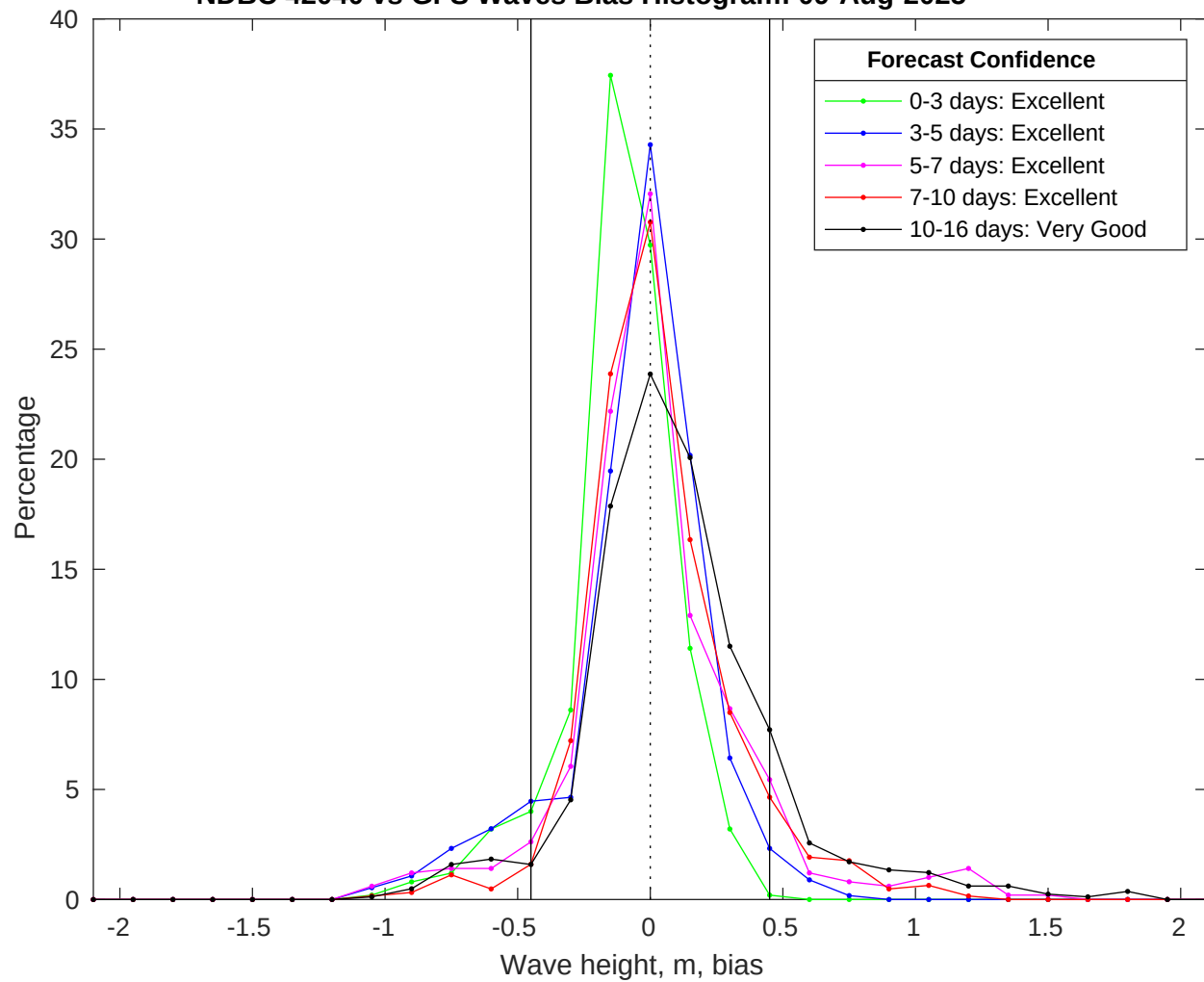
NDBC 42040 vs GFS Waves Bias Histogram: 09-Aug-2025
