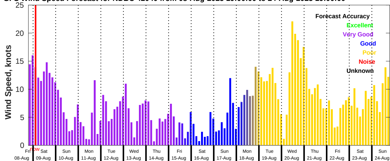
GFS Wind Speed Forecast for NDBC 42040 from 08-Aug-2025 19:00:00 to 24-Aug-2025 19:00:00
