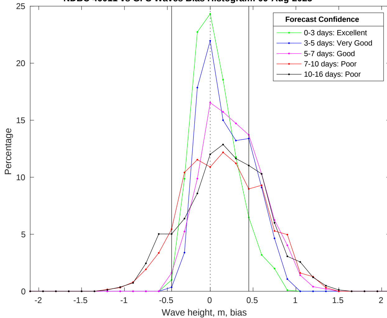
NDBC 46011 vs GFS Waves Bias Histogram: 09-Aug-2025
