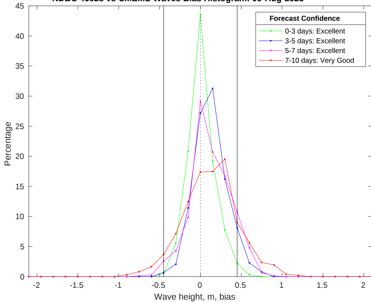
NDBC 46028 vs CMEMS Waves Bias Histogram: 09-Aug-2025
