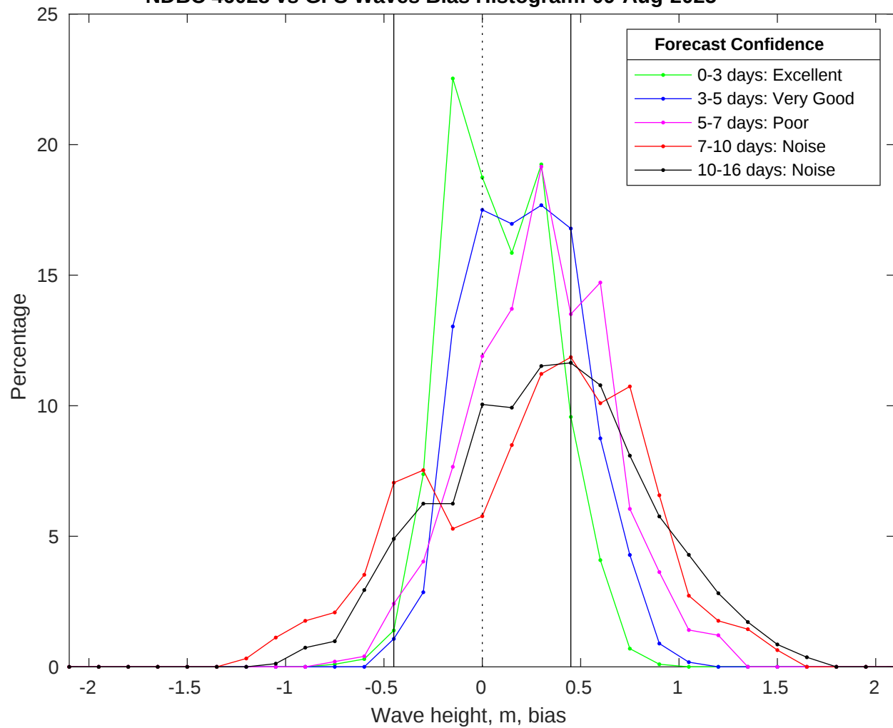
NDBC 46028 vs GFS Waves Bias Histogram: 09-Aug-2025
