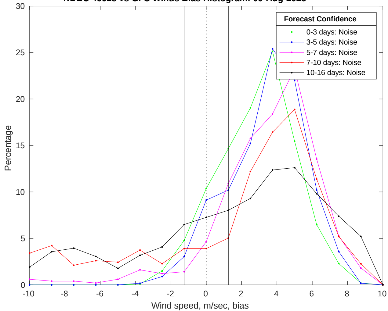
NDBC 46028 vs GFS Winds Bias Histogram: 09-Aug-2025
