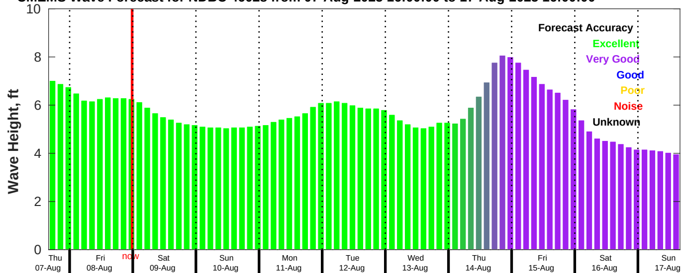
CMEMS Wave Forecast for NDBC 46028 from 07-Aug-2025 16:00:00 to 17-Aug-2025 16:00:00
