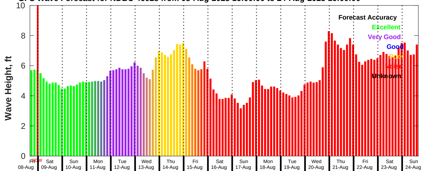
GFS Wave Forecast for NDBC 46028 from 08-Aug-2025 16:00:00 to 24-Aug-2025 16:00:00
