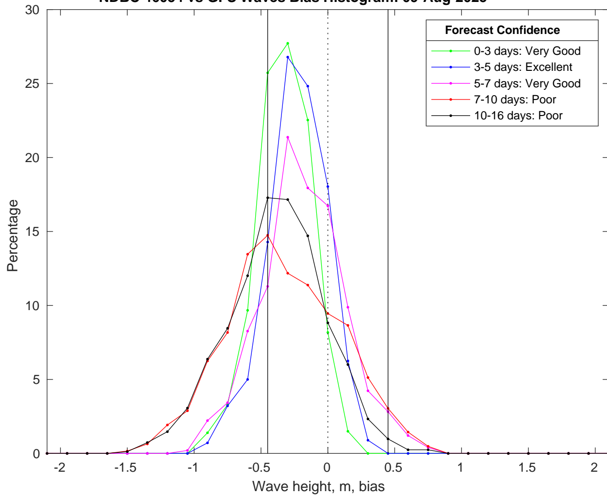
NDBC 46054 vs GFS Waves Bias Histogram: 09-Aug-2025
