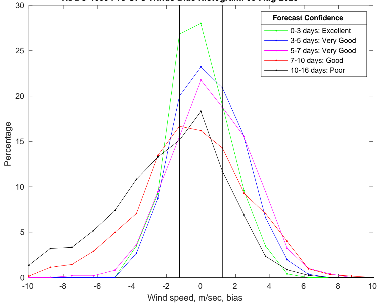
NDBC 46054 vs GFS Winds Bias Histogram: 09-Aug-2025
