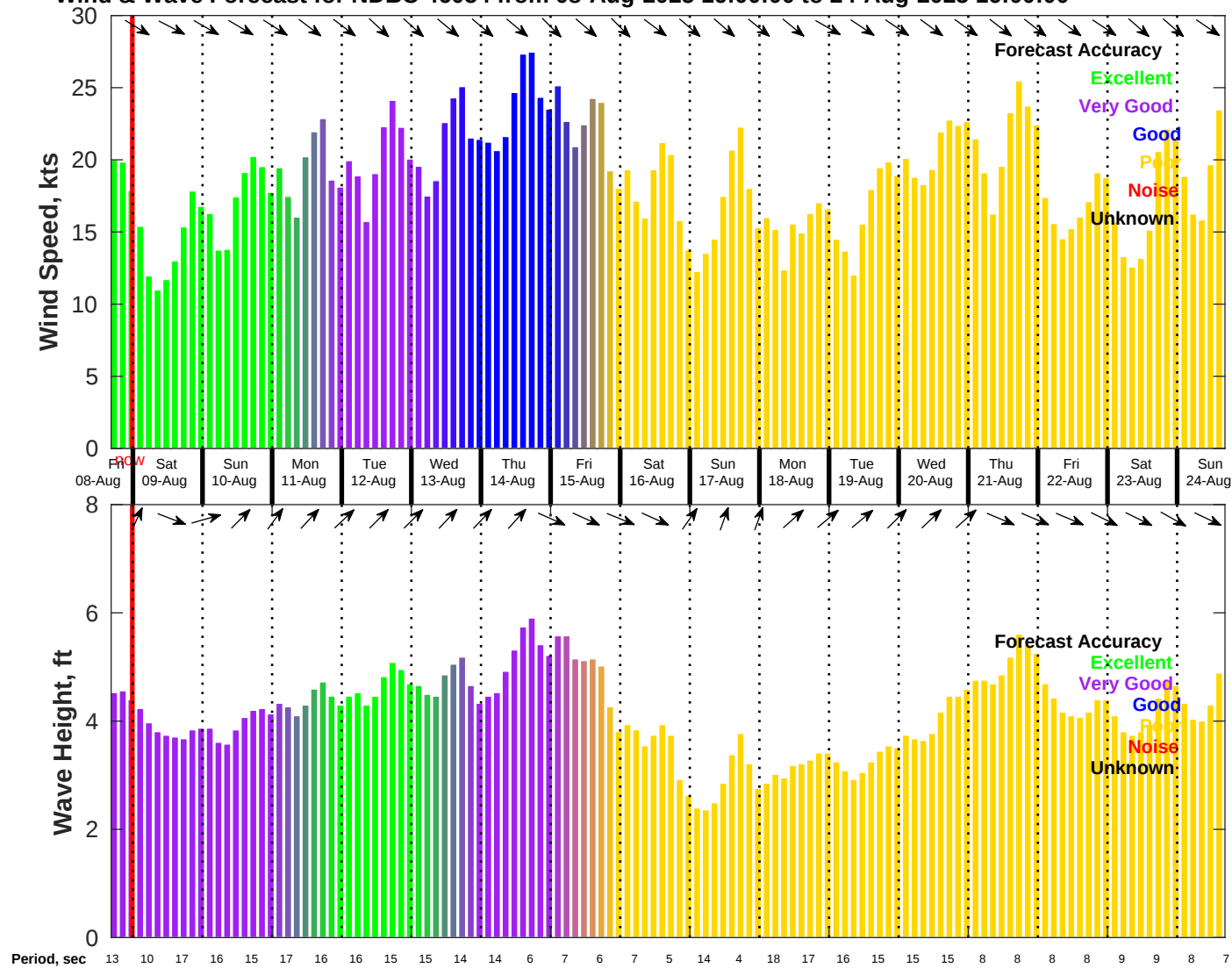
Wind & Wave Forecast for NDBC 46054 from 08-Aug-2025 16:00:00 to 24-Aug-2025 16:00:00
