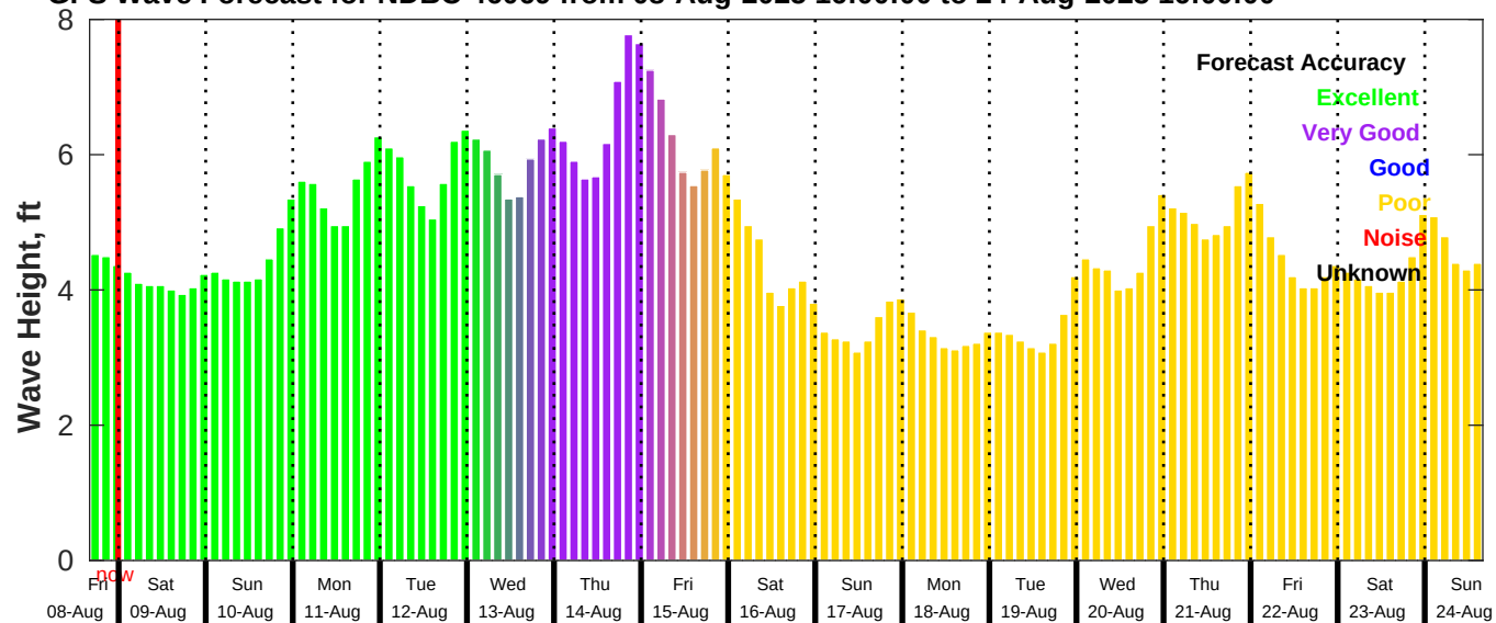
GFS Wave Forecast for NDBC 46069 from 08-Aug-2025 16:00:00 to 24-Aug-2025 16:00:00
