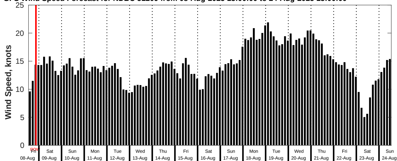
GFS Wind Speed Forecast for NDBC 51209 from 08-Aug-2025 13:00:00 to 24-Aug-2025 13:00:00
