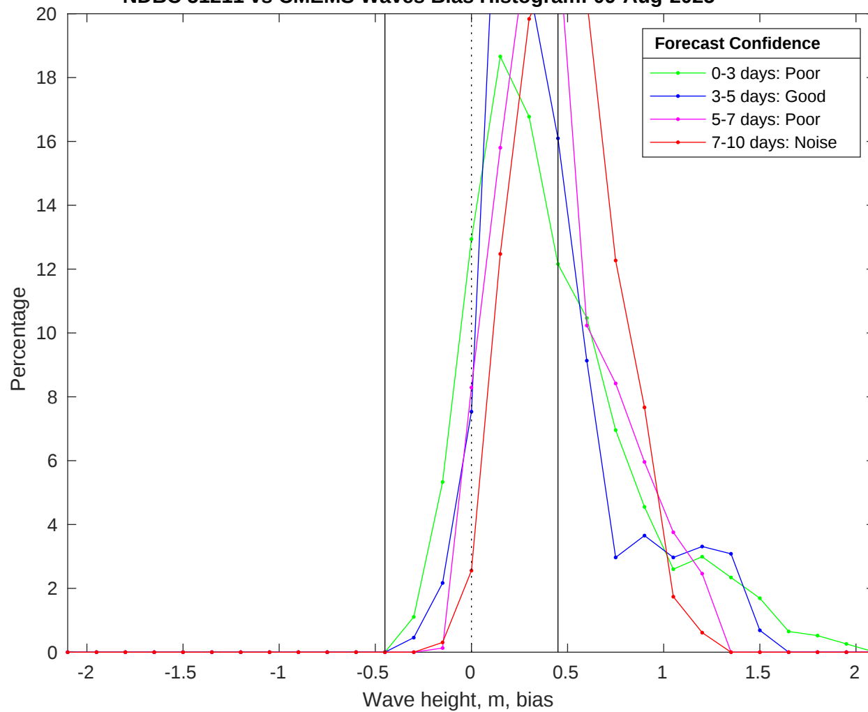
NDBC 51211 vs CMEMS Waves Bias Histogram: 09-Aug-2025
