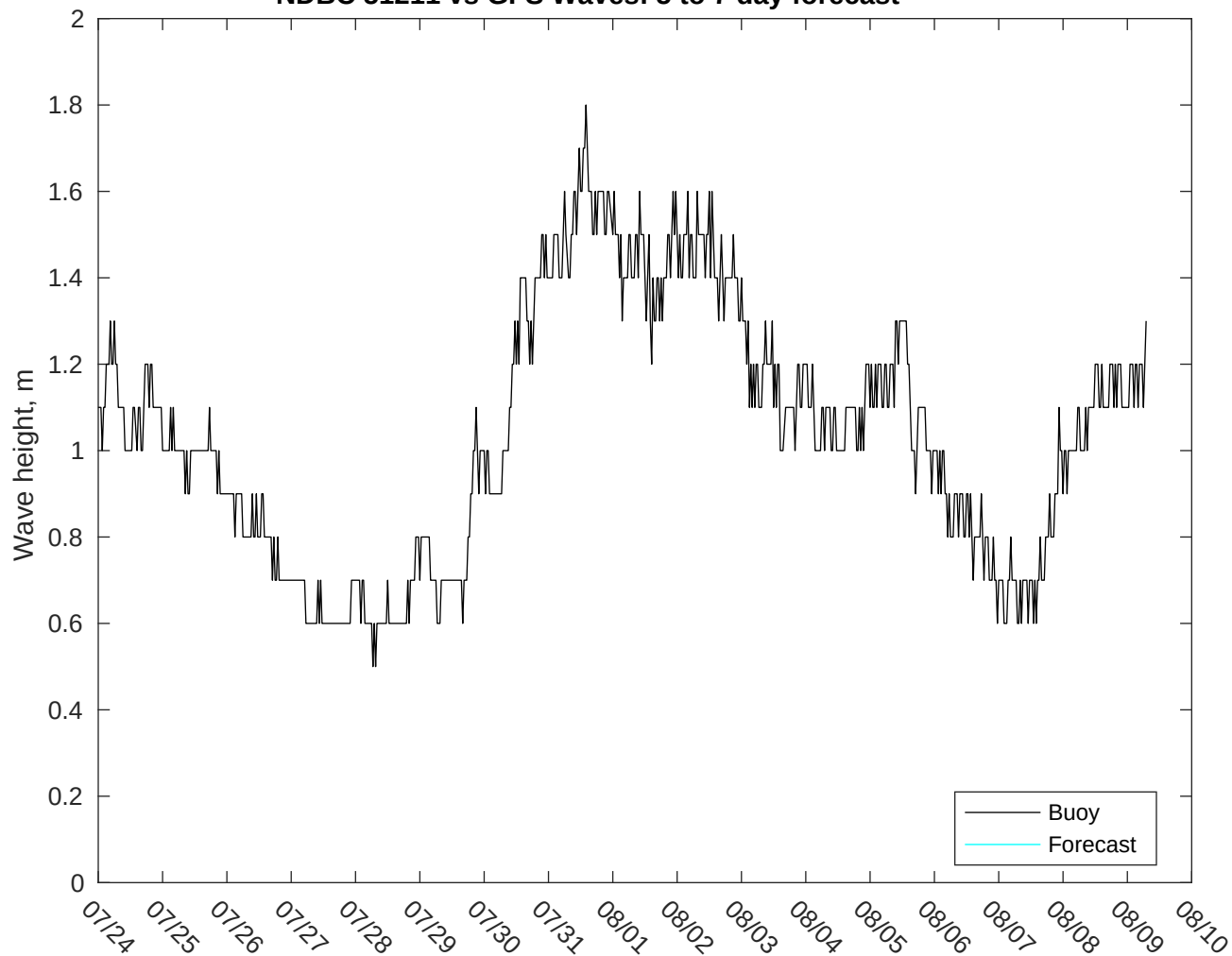
NDBC 51211 vs GFS Waves: 5 to 7 day forecast
