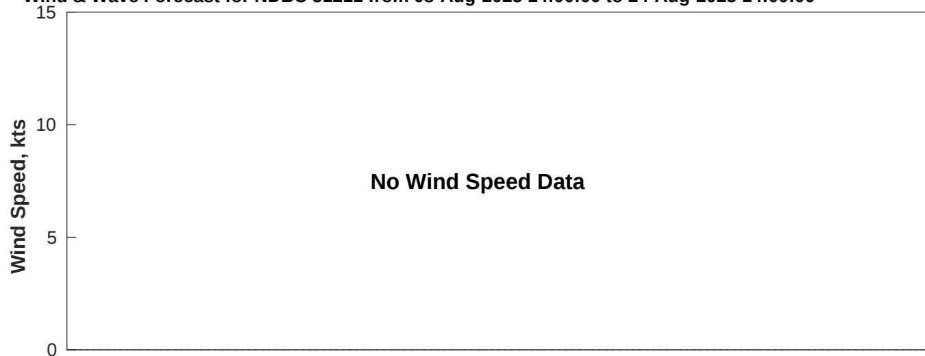
Wind & Wave Forecast for NDBC 51211 from 08-Aug-2025 14:00:00 to 24-Aug-2025 14:00:00
