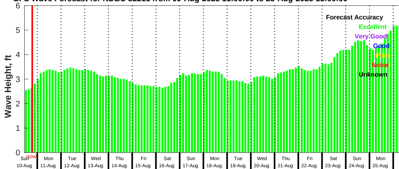
GFS Wave Forecast for NDBC 52211 from 09-Aug-2025 11:00:00 to 25-Aug-2025 11:00:00
