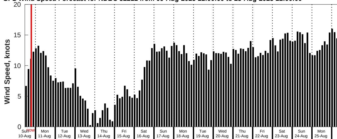
GFS Wind Speed Forecast for NDBC 52211 from 09-Aug-2025 11:00:00 to 25-Aug-2025 11:00:00
