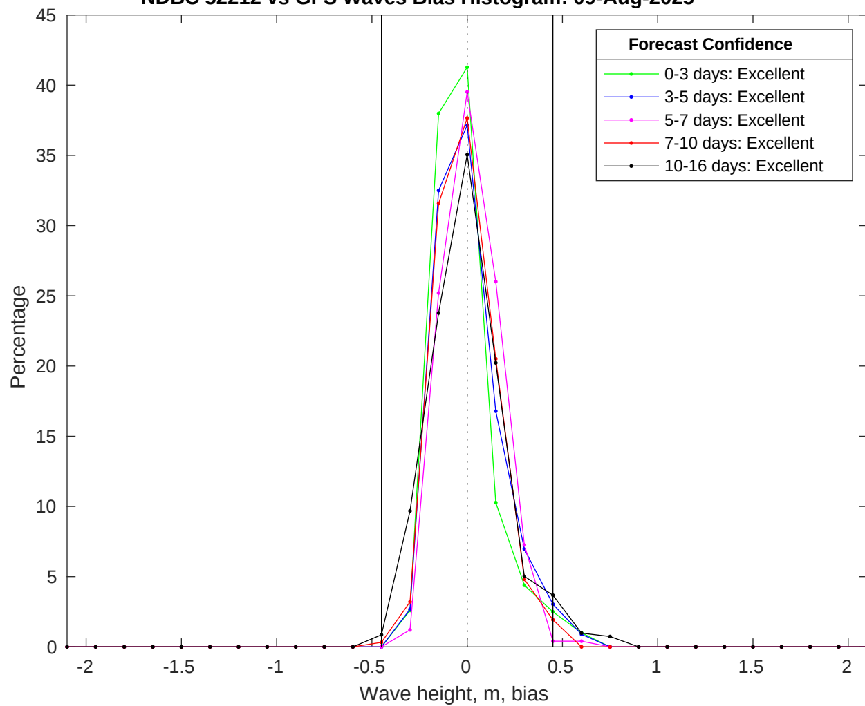
NDBC 52212 vs GFS Waves Bias Histogram: 09-Aug-2025
