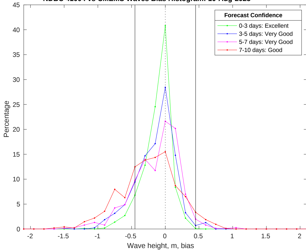
NDBC 41004 vs CMEMS Waves Bias Histogram: 10-Aug-2025
