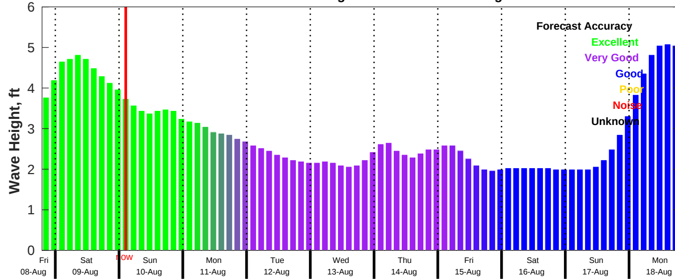
CMEMS Wave Forecast for NDBC 41004 from 08-Aug-2025 19:00:00 to 18-Aug-2025 19:00:00
