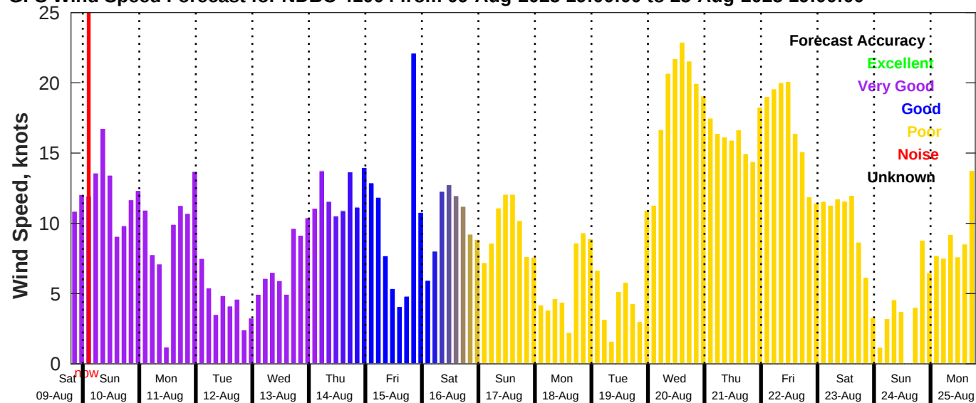
GFS Wind Speed Forecast for NDBC 41004 from 09-Aug-2025 19:00:00 to 25-Aug-2025 19:00:00
