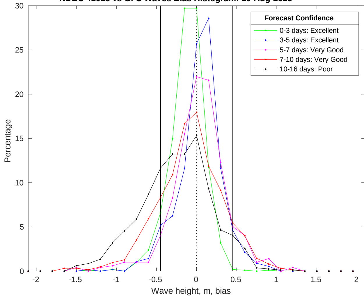
NDBC 41013 vs GFS Waves Bias Histogram: 10-Aug-2025
