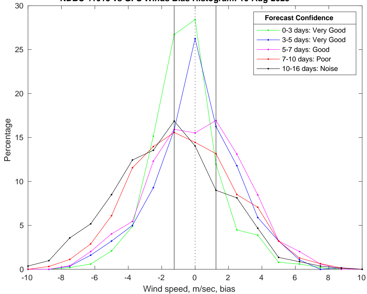
NDBC 41013 vs GFS Winds Bias Histogram: 10-Aug-2025
