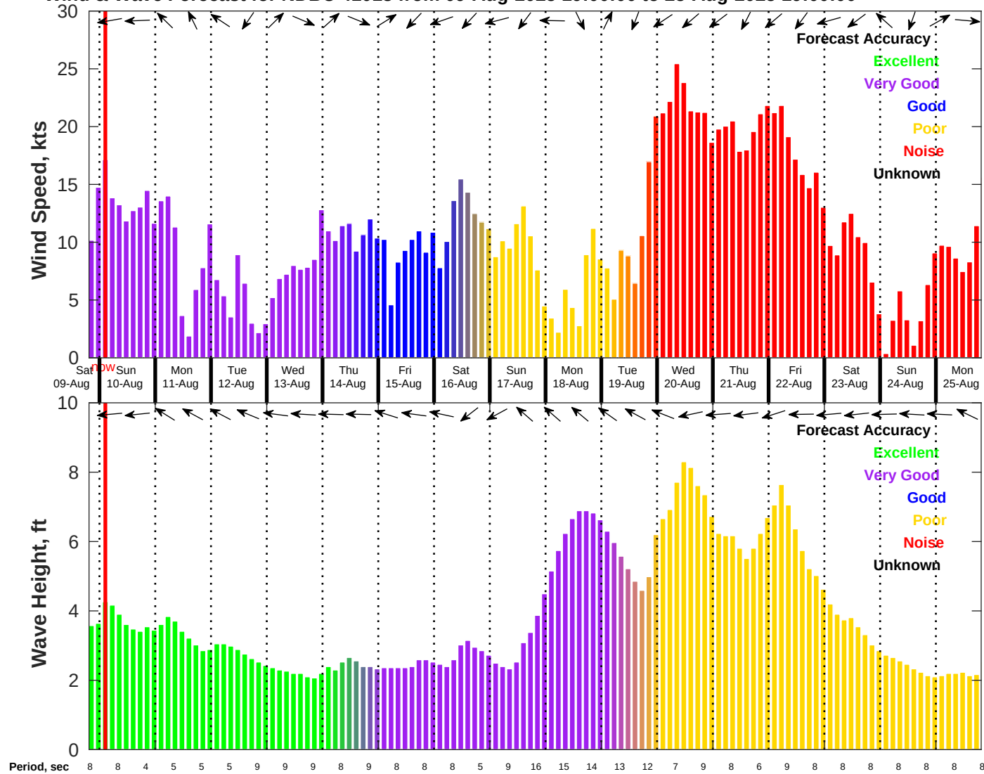
Wind & Wave Forecast for NDBC 41013 from 09-Aug-2025 19:00:00 to 25-Aug-2025 19:00:00
