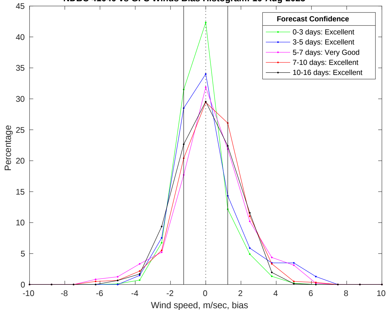
NDBC 41040 vs GFS Winds Bias Histogram: 10-Aug-2025
