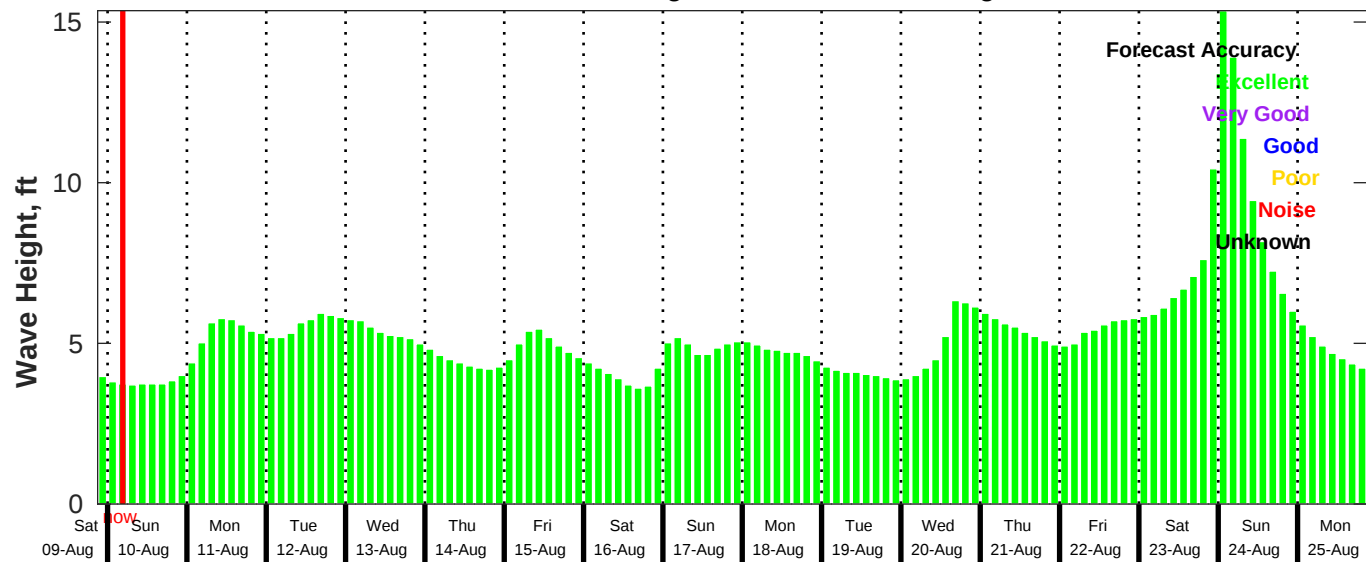
GFS Wave Forecast for NDBC 41040 from 09-Aug-2025 21:00:00 to 25-Aug-2025 21:00:00
