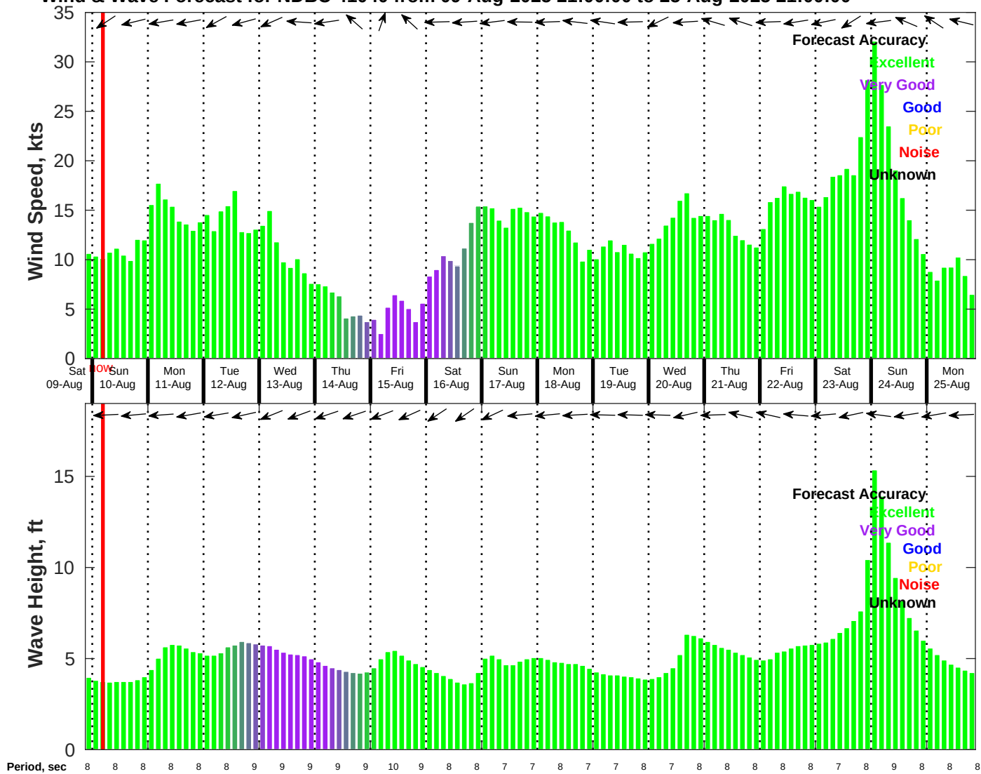
Wind & Wave Forecast for NDBC 41040 from 09-Aug-2025 21:00:00 to 25-Aug-2025 21:00:00
