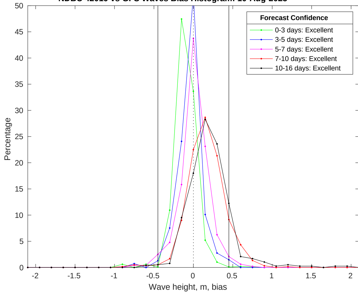
NDBC 42019 vs GFS Waves Bias Histogram: 10-Aug-2025
