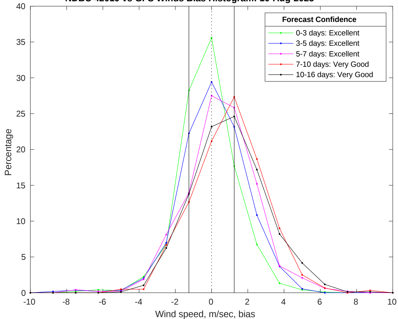
NDBC 42019 vs GFS Winds Bias Histogram: 10-Aug-2025
