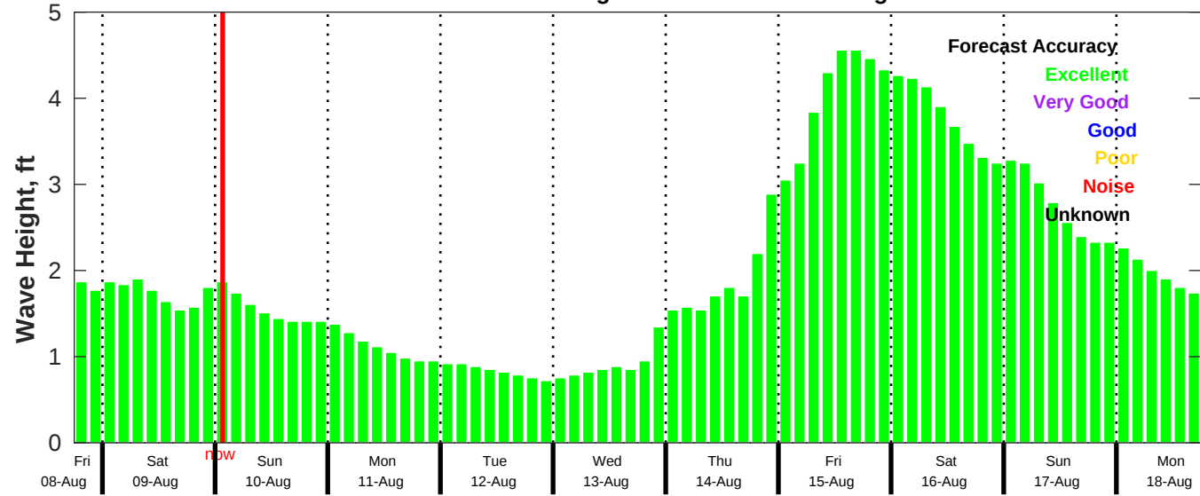
CMEMS Wave Forecast for NDBC 42019 from 08-Aug-2025 18:00:00 to 18-Aug-2025 18:00:00
