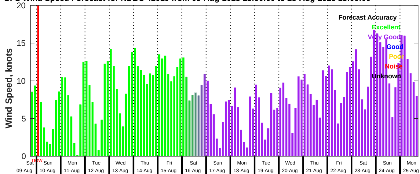
GFS Wind Speed Forecast for NDBC 42019 from 09-Aug-2025 18:00:00 to 25-Aug-2025 18:00:00
