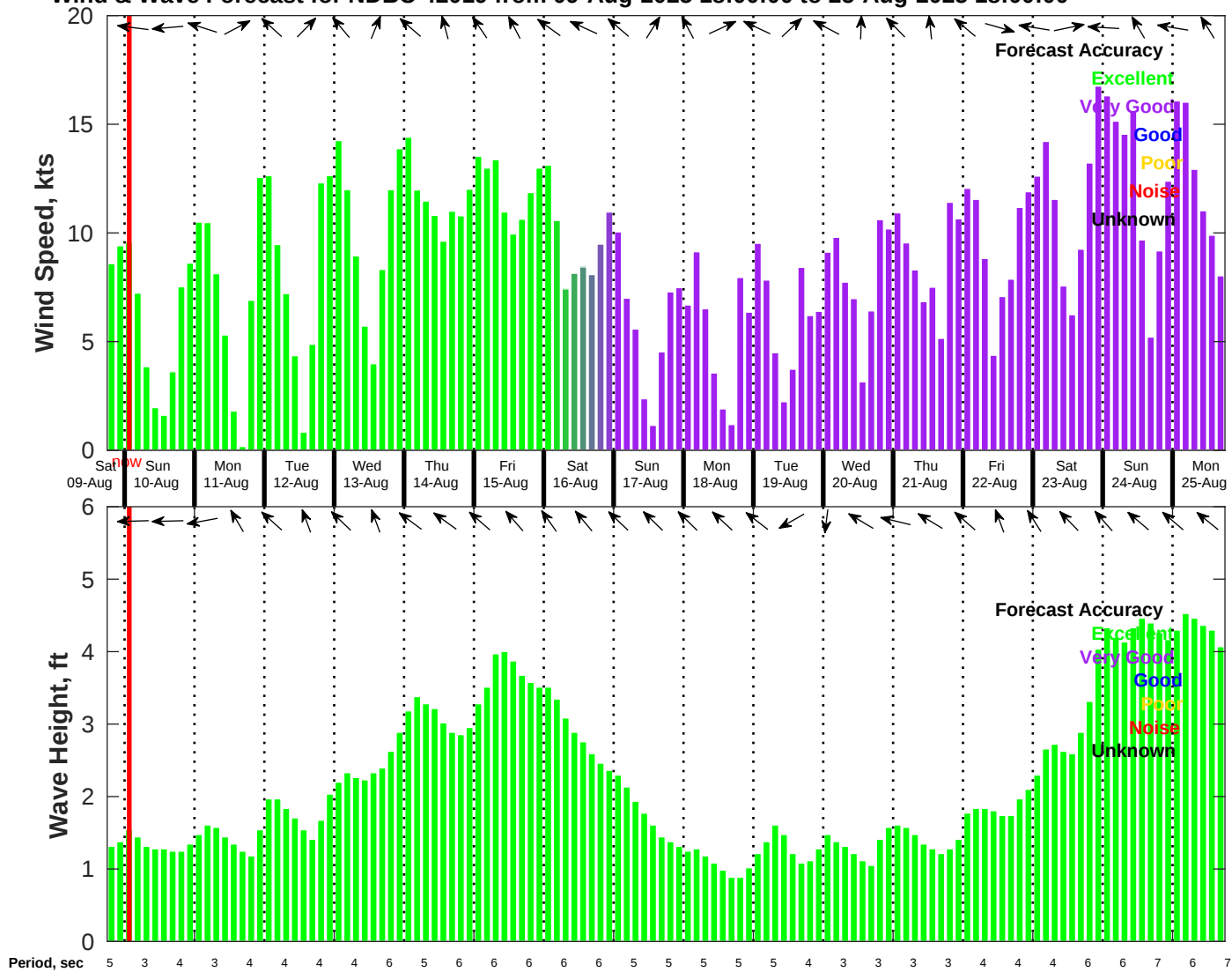
Wind & Wave Forecast for NDBC 42019 from 09-Aug-2025 18:00:00 to 25-Aug-2025 18:00:00
