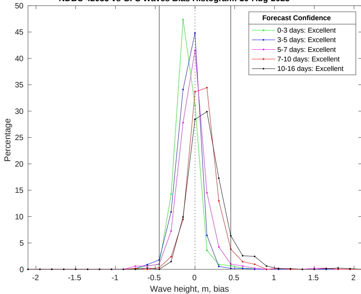
NDBC 42035 vs GFS Waves Bias Histogram: 10-Aug-2025
