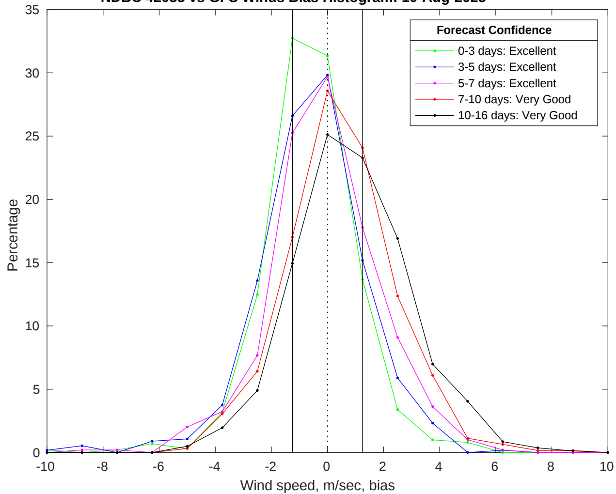
NDBC 42035 vs GFS Winds Bias Histogram: 10-Aug-2025
