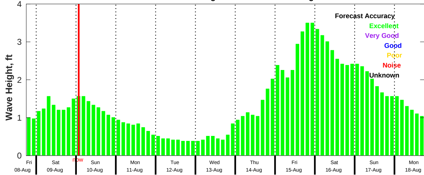
CMEMS Wave Forecast for NDBC 42035 from 08-Aug-2025 18:00:00 to 18-Aug-2025 18:00:00
