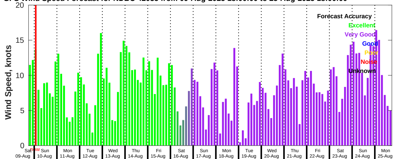
GFS Wind Speed Forecast for NDBC 42035 from 09-Aug-2025 18:00:00 to 25-Aug-2025 18:00:00
