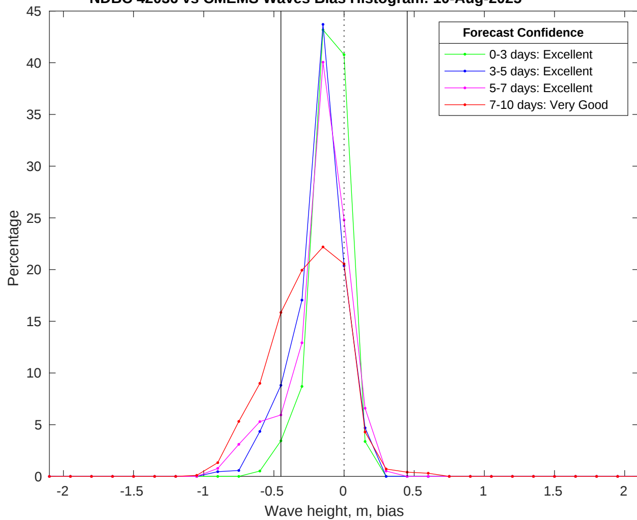
NDBC 42036 vs CMEMS Waves Bias Histogram: 10-Aug-2025
