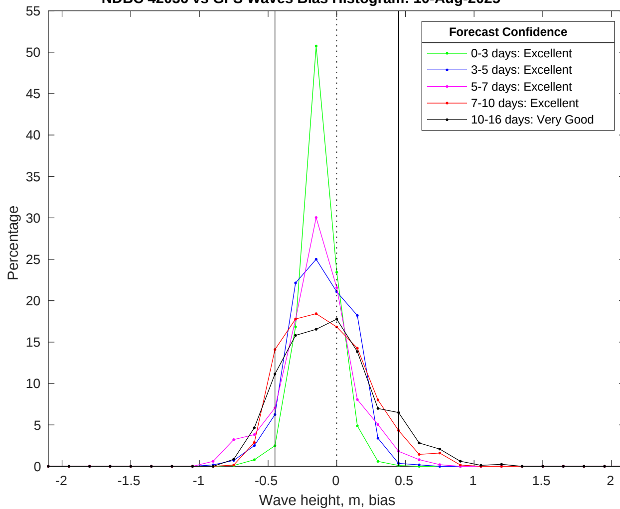
NDBC 42036 vs GFS Waves Bias Histogram: 10-Aug-2025
