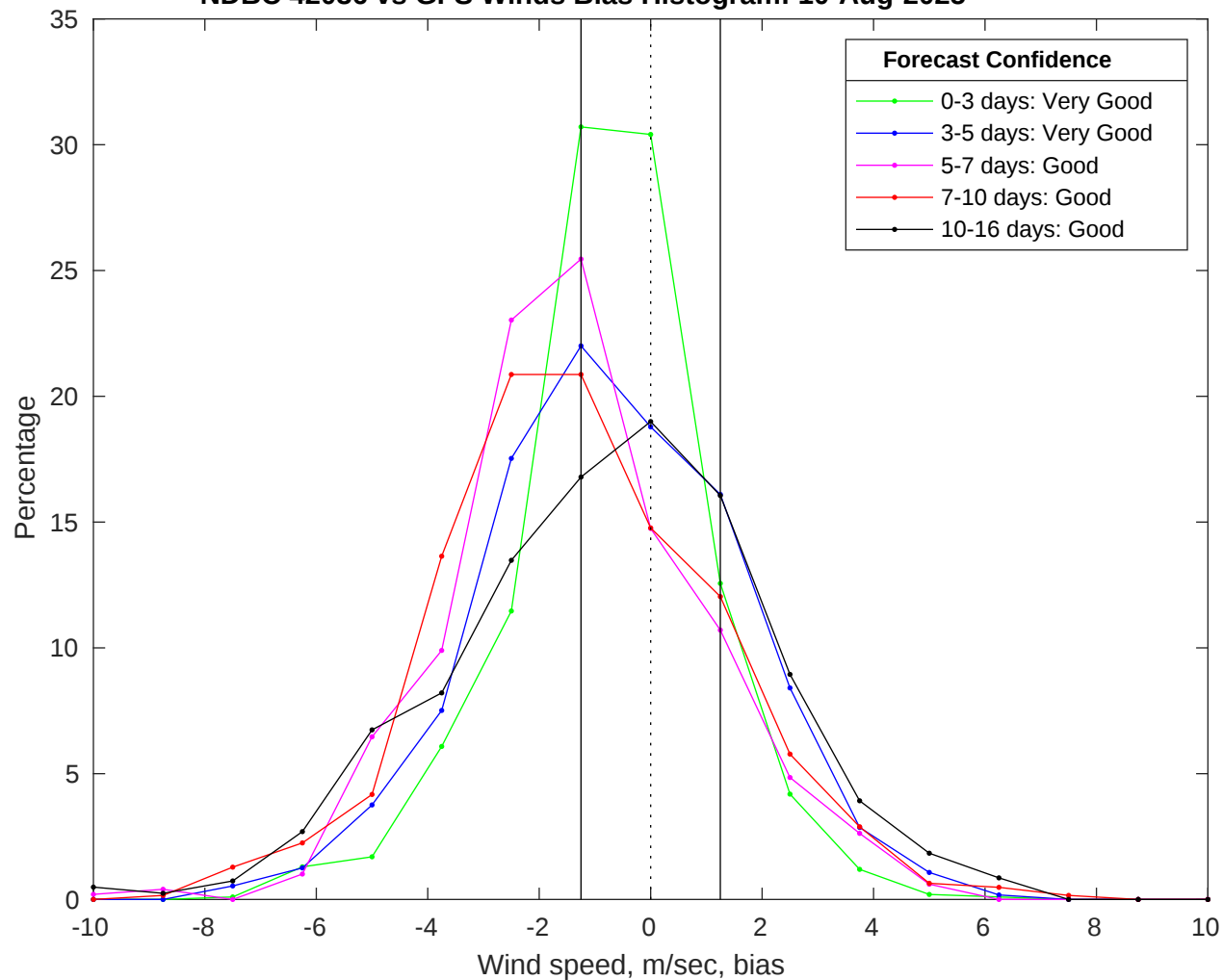
NDBC 42036 vs GFS Winds Bias Histogram: 10-Aug-2025
