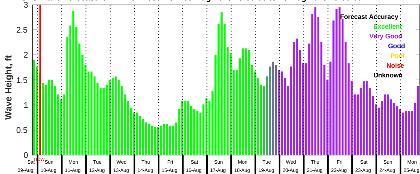
GFS Wave Forecast for NDBC 42036 from 09-Aug-2025 19:00:00 to 25-Aug-2025 19:00:00
