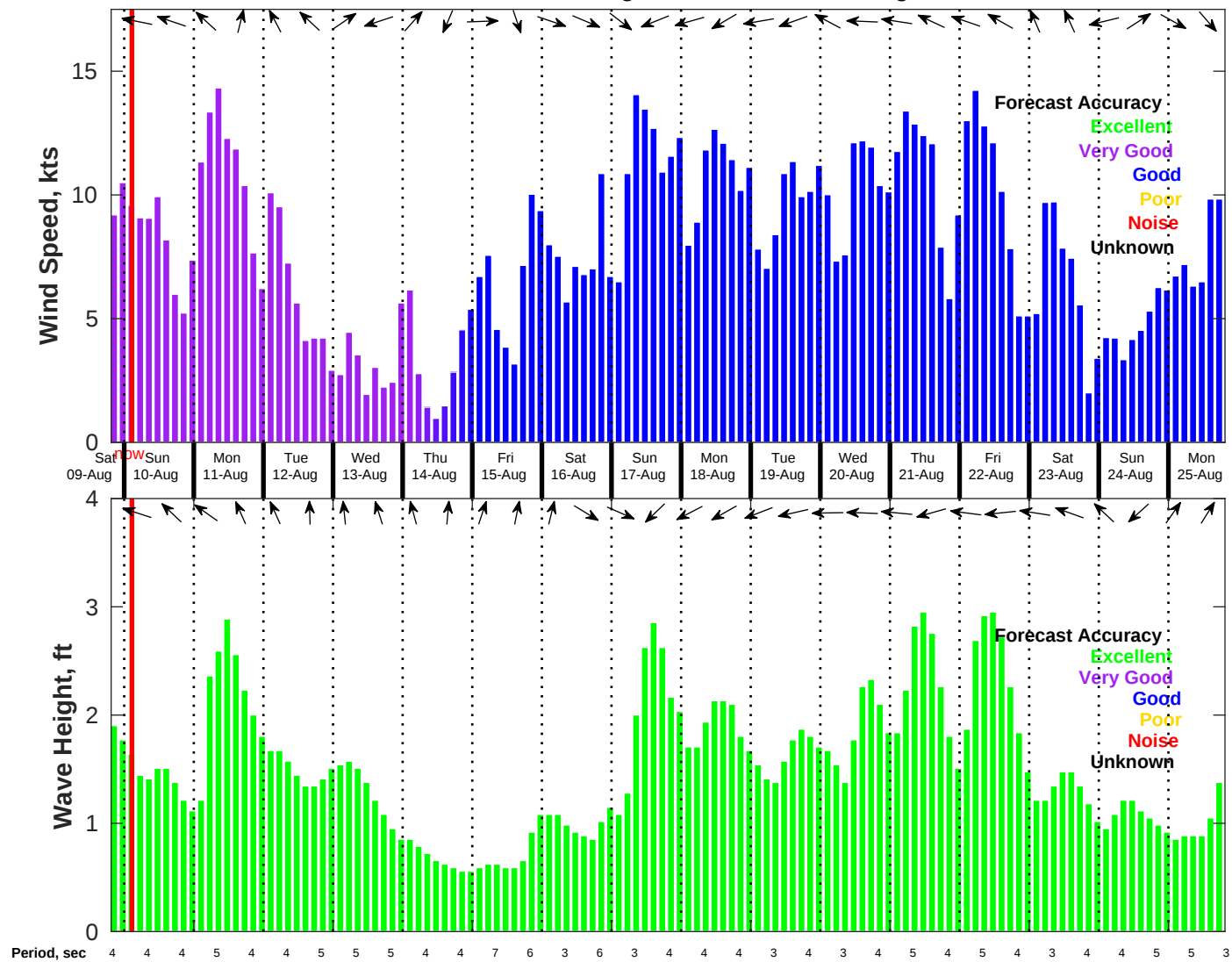
Wind & Wave Forecast for NDBC 42036 from 09-Aug-2025 19:00:00 to 25-Aug-2025 19:00:00
