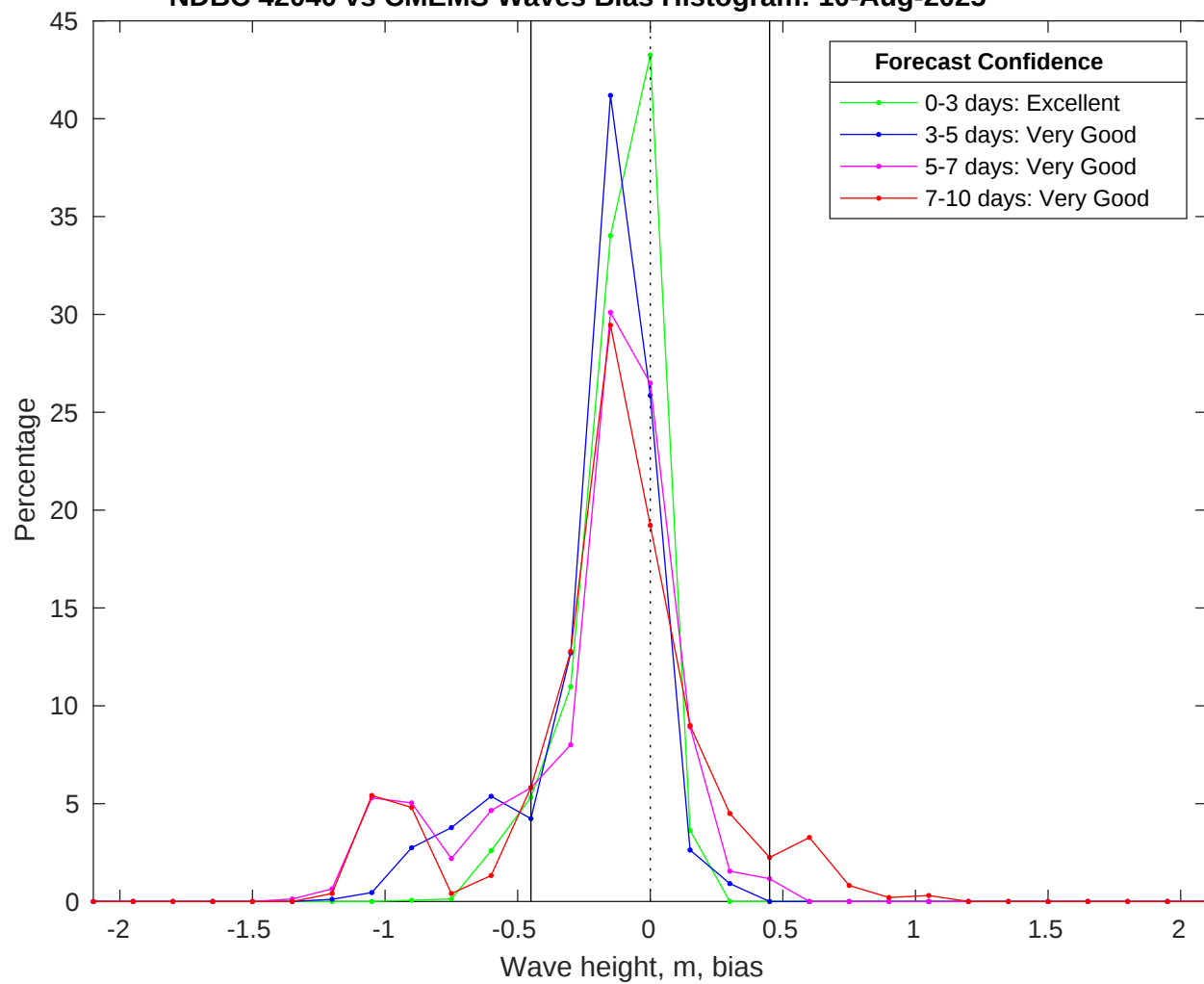
NDBC 42040 vs CMEMS Waves Bias Histogram: 10-Aug-2025
