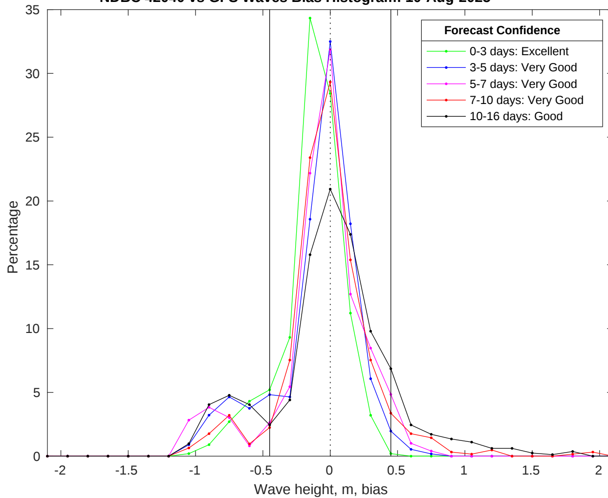
NDBC 42040 vs GFS Waves Bias Histogram: 10-Aug-2025
