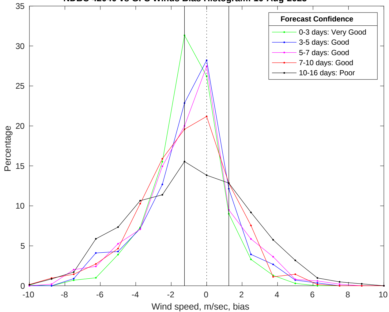
NDBC 42040 vs GFS Winds Bias Histogram: 10-Aug-2025
