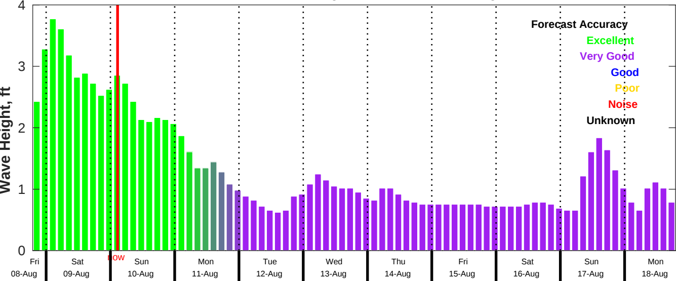
CMEMS Wave Forecast for NDBC 42040 from 08-Aug-2025 19:00:00 to 18-Aug-2025 19:00:00
