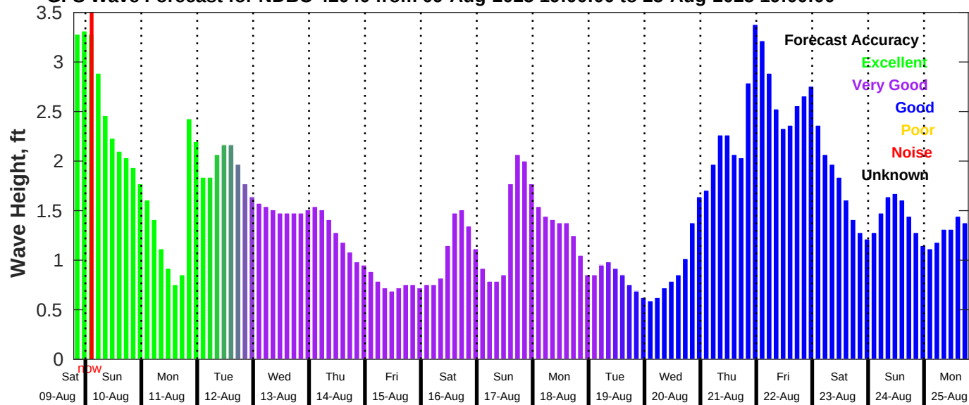
GFS Wave Forecast for NDBC 42040 from 09-Aug-2025 19:00:00 to 25-Aug-2025 19:00:00
