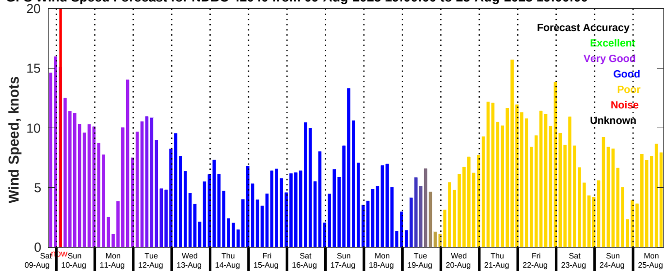
GFS Wind Speed Forecast for NDBC 42040 from 09-Aug-2025 19:00:00 to 25-Aug-2025 19:00:00
