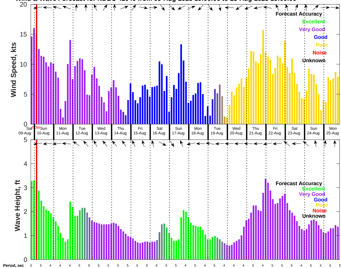
Wind & Wave Forecast for NDBC 42040 from 09-Aug-2025 19:00:00 to 25-Aug-2025 19:00:00
